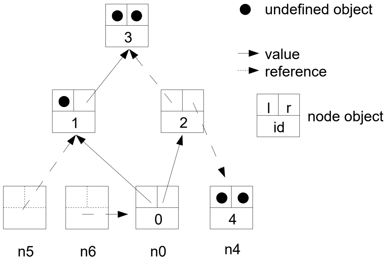
Figure 1: Graph model
