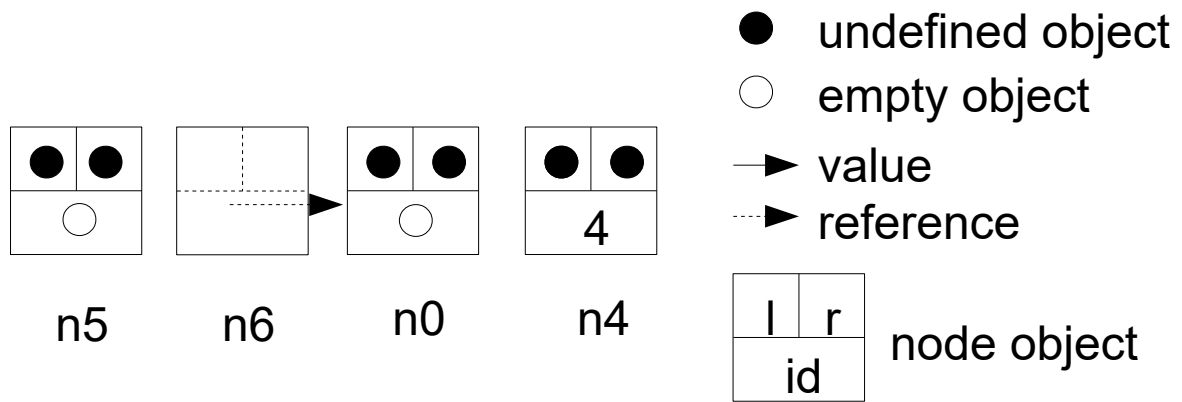
Figure 2: Graph model after clearing n0
